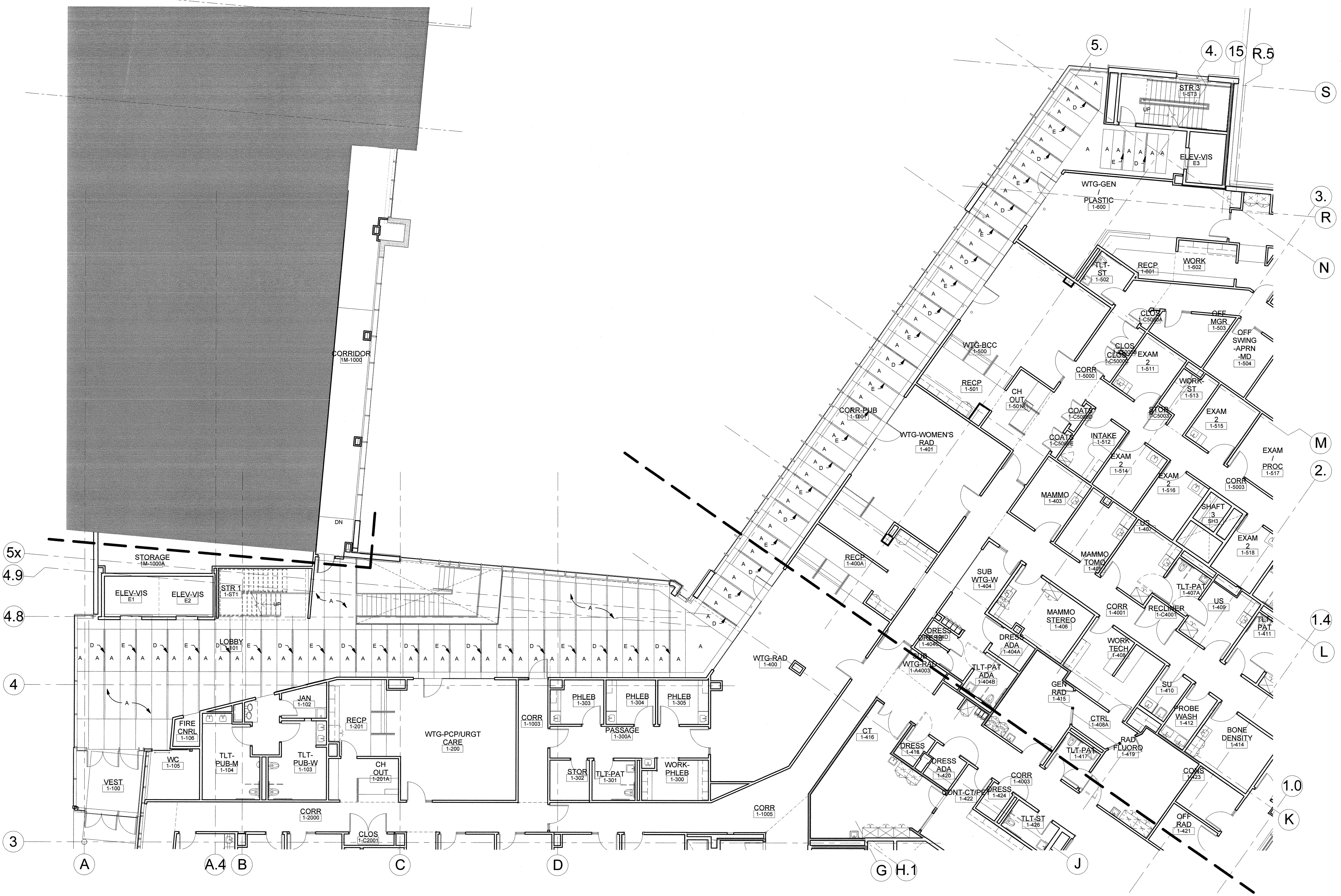
1 1-101 LOBBY FLOOR FINISH PLAN 1/8" = 1'-0"
