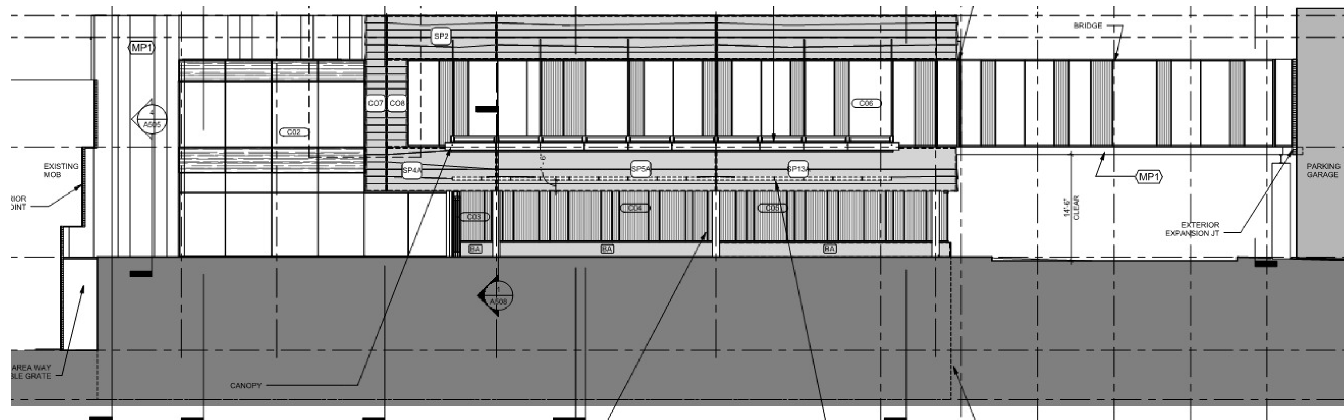
BRIDGE CORRIDOR EXTERIOR ELEVATION
