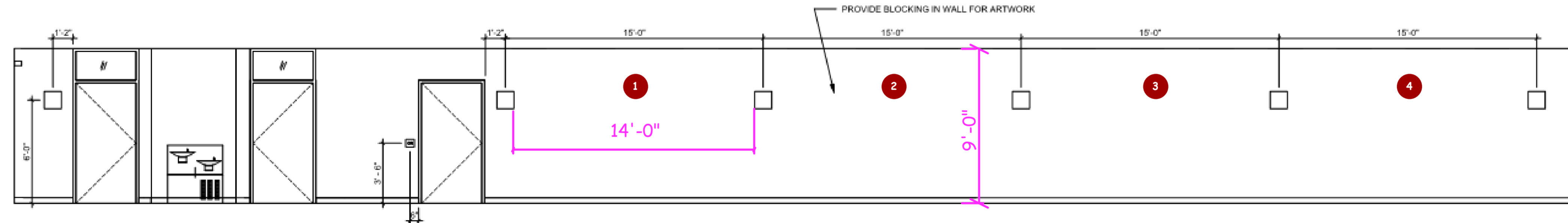
BRIDGE CORRIDOR INTERIOR ELEVATION
