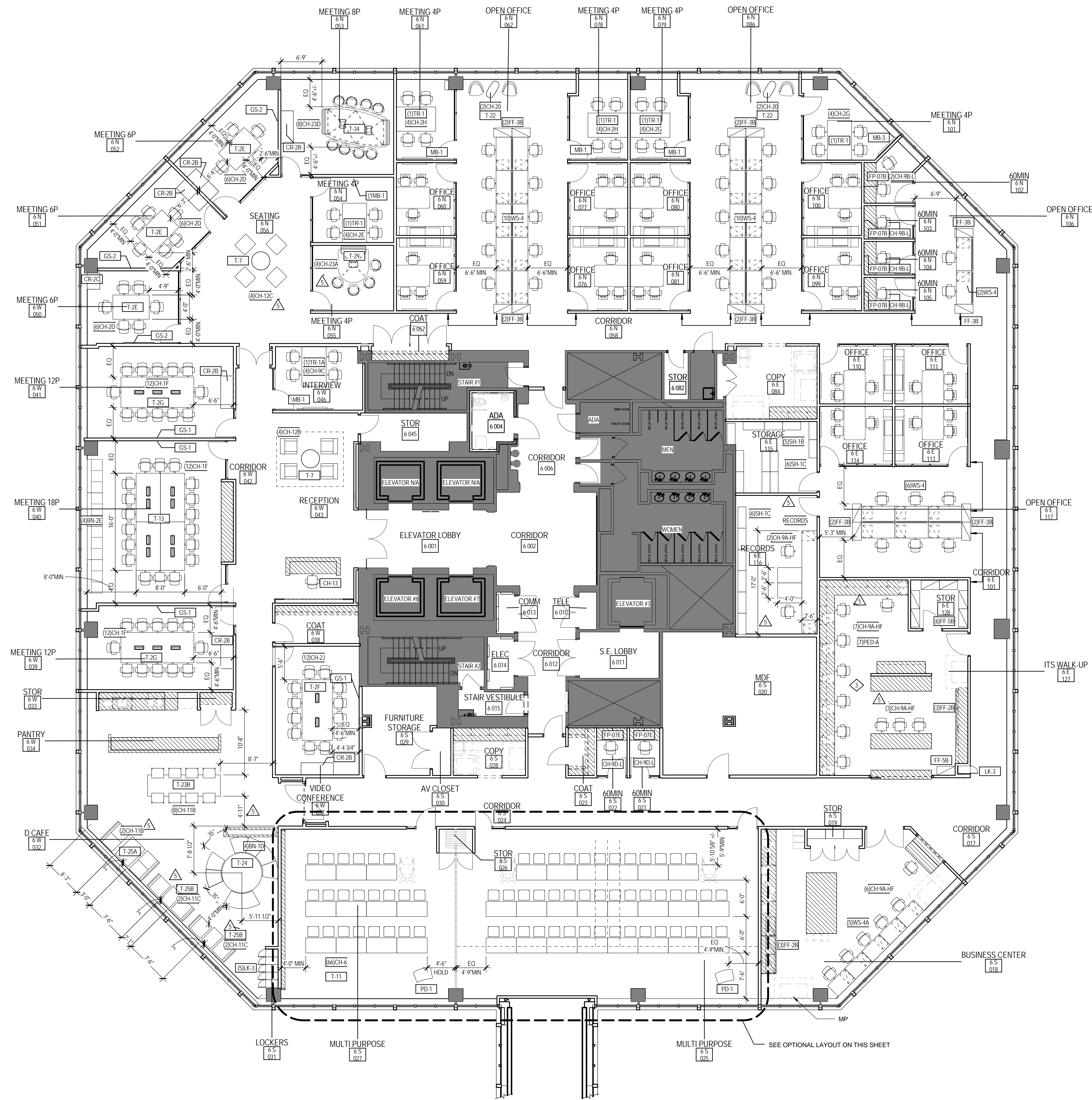
1 FURNITURE PLAN - LEVEL 6 1/8" = 1'-0"
