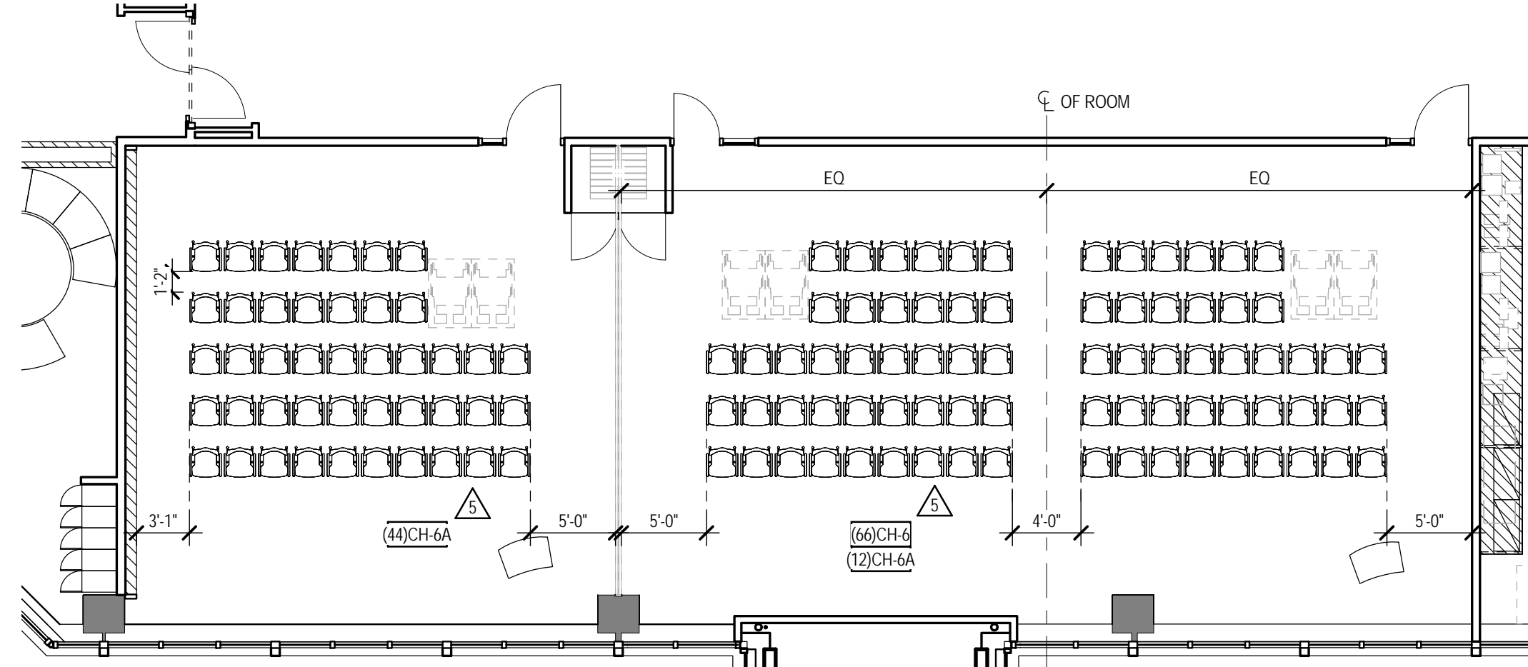
4 MP ROOM-DCE LAYOUT - FURNITURE PLAN 1/8" = 1'-0"
