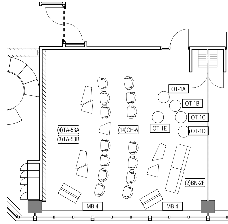
4 MP ROOM-DCE LAYOUT - FURNITURE PLAN 1/8" = 1'-0"
